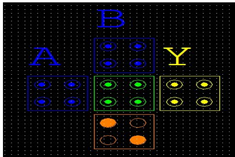
Figure 5: AND gate implementation using QCA
