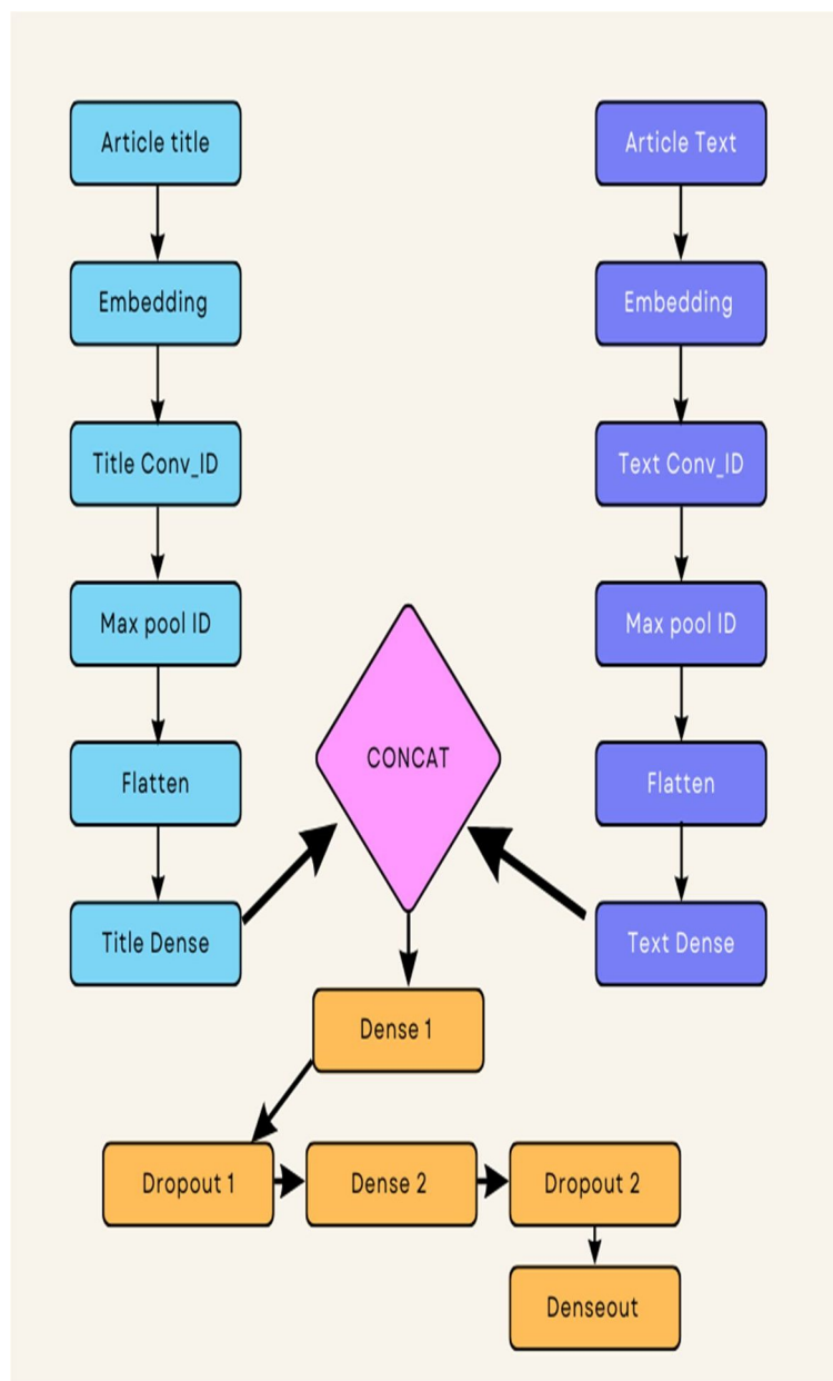
Fig 3: 7 Layer CNN architecture.
