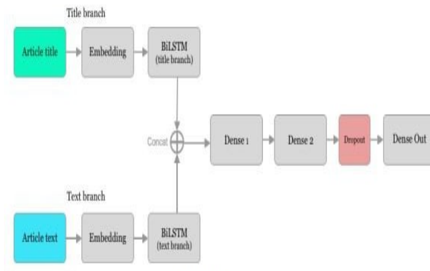
Fig 2: LSTM architecture workflow.
