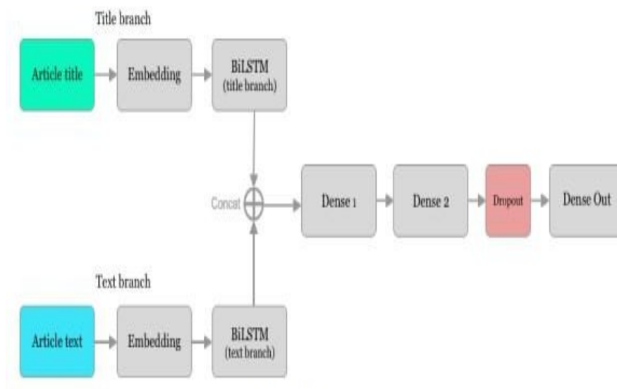
Fig 2: LSTM architecture workflow.
